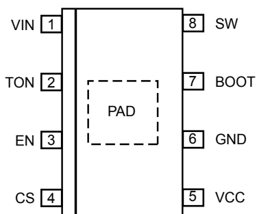
Pinout Diagram
